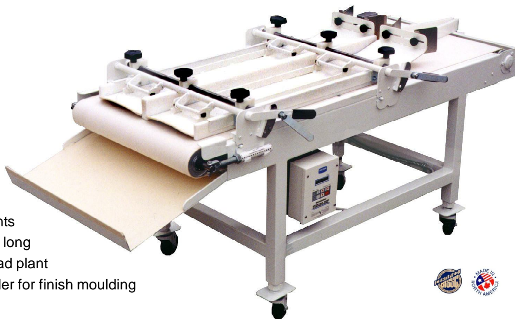
SIMPLEX 24B c/w variable speed, optional dual pressure plates and side guides shown
